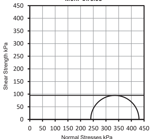
Mohr Circles
