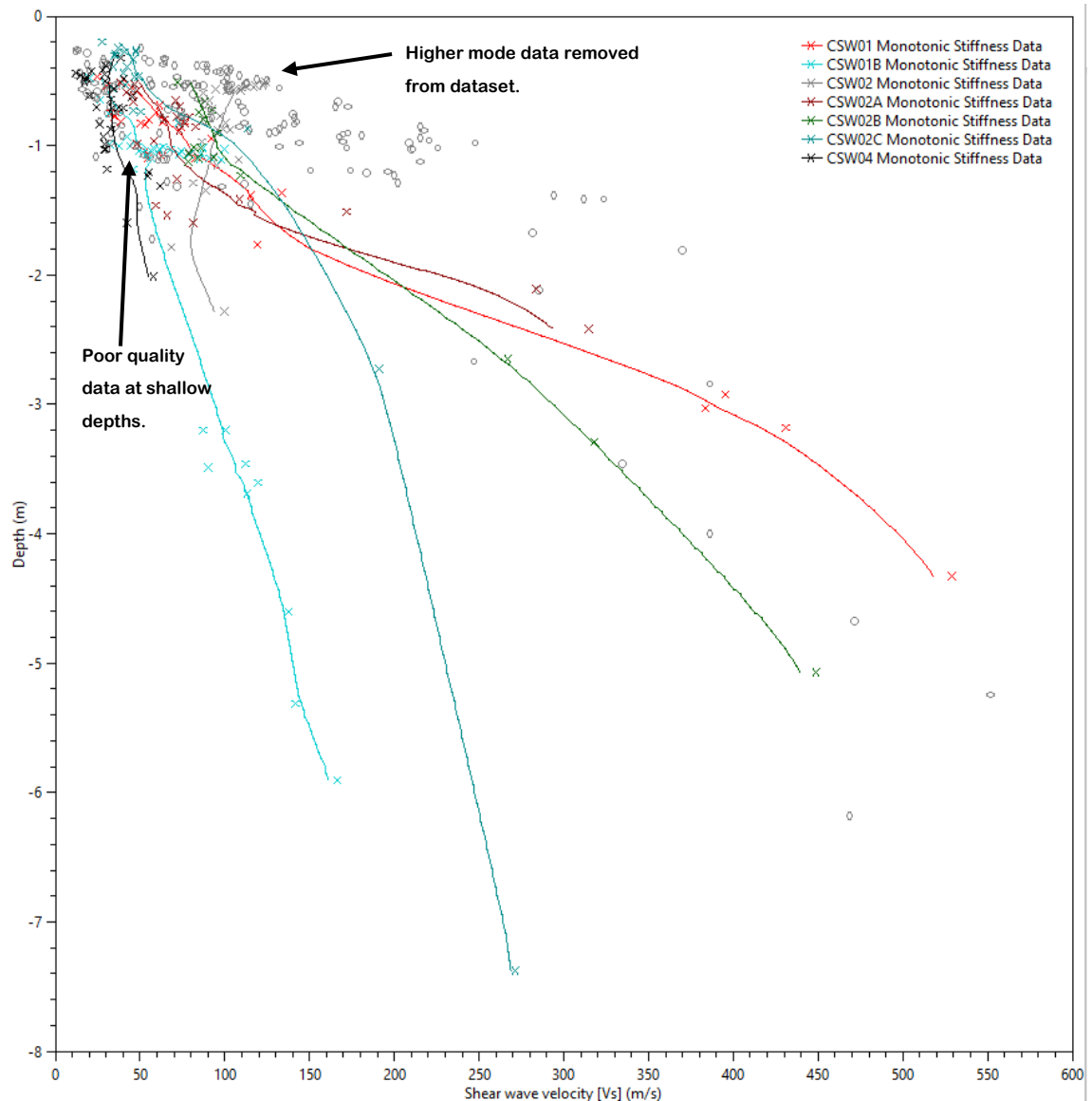
Figure 5-1: Superimposed graph showing simple inversions of ACSW tests CSW01, 01B, 02, 02A, 02B, 02C & 04.
