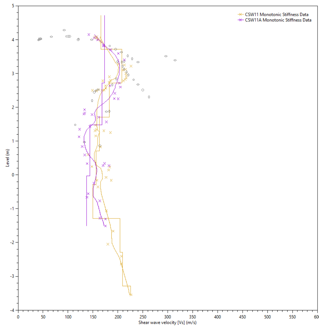
Figure 5-3: Simple and Advanced inversions for CSW11 and CSW11A.
