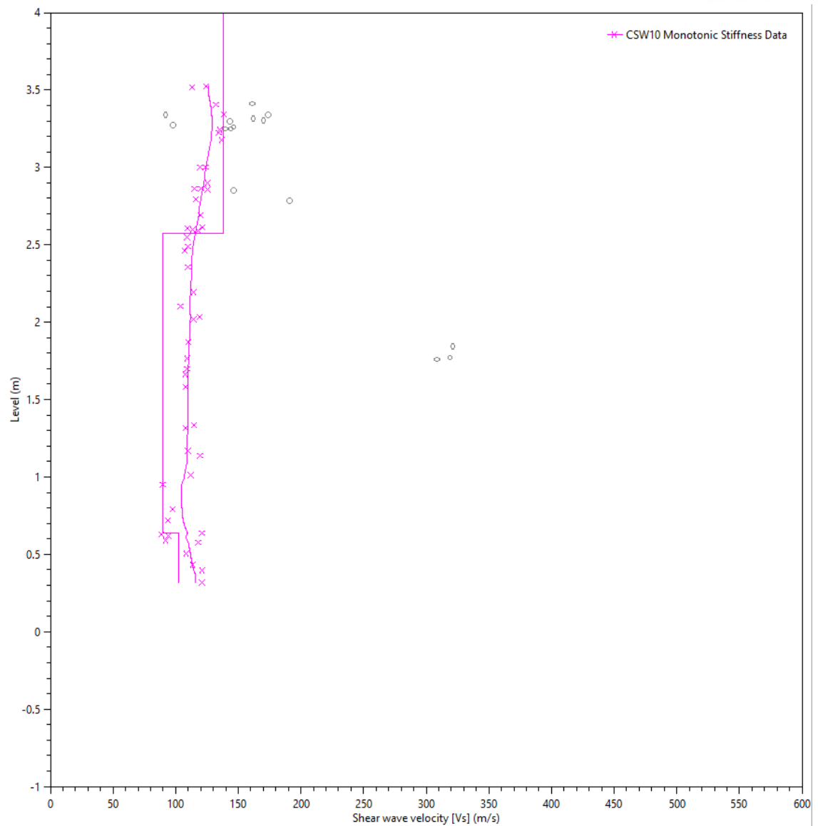
Figure 5-2: Simple and Advanced Inversions of CSW10.
